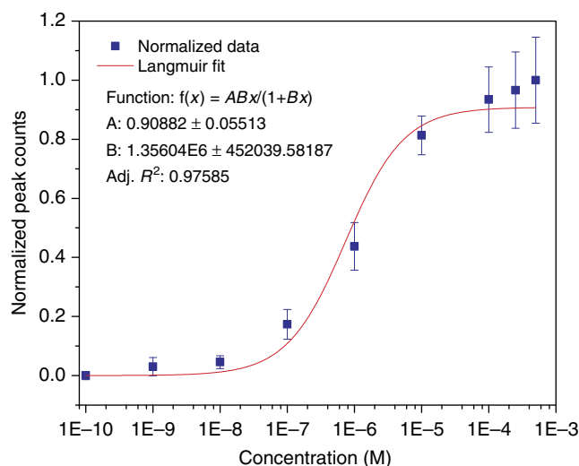
Figure 2 | Count rates as a function of concentration. Plot of normalized RT counting rates vs concentration of \alpha -M 1 Glu for trapping the analyte in an RT gap functionalized with ICA molecules and a fit to a Langmuir isotherm.
